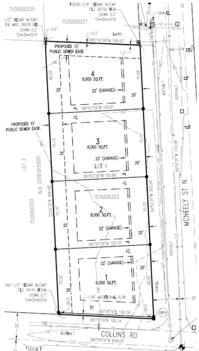
Survey Drawing of Proposed Short Plat
